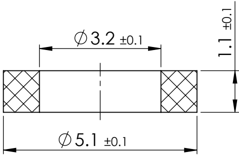
SECTION X-X
